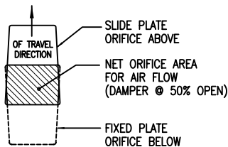
3 ORIFICE DETAIL
