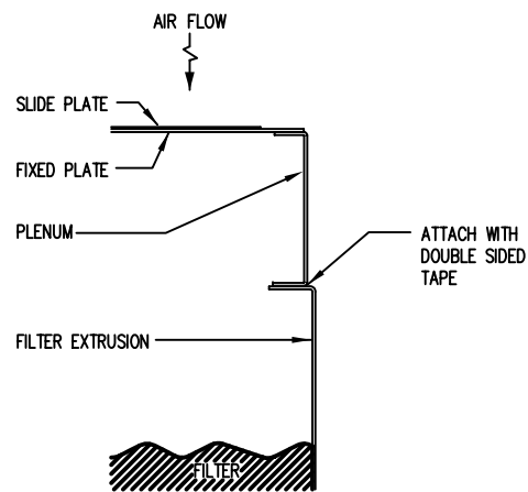
5 ENLARGED DETAIL
