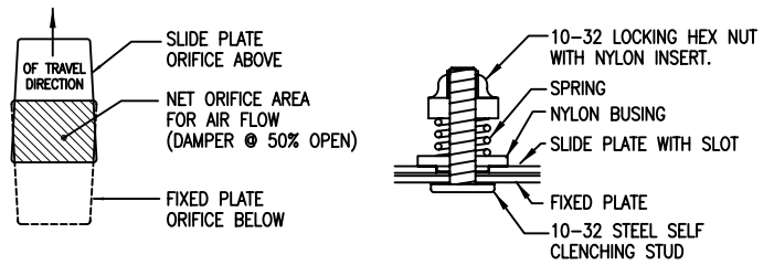
3 ORIFICE DETAIL
