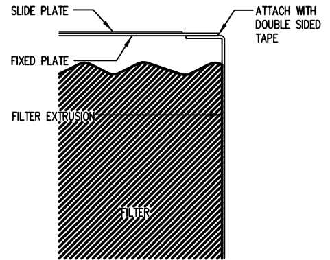
5 ENLARGED DETAIL
