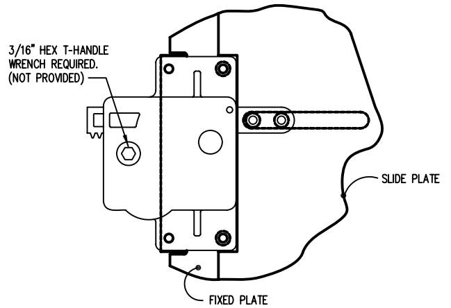
2 DAMPER ADJUSTMENT ASSEMBLY
