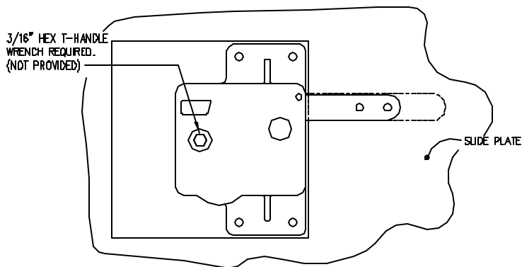
2 DAMPER ADJUSTMENT ASSEMBLY
