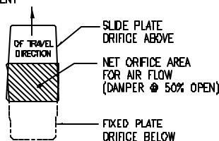
3 ORIFICE DETAIL
