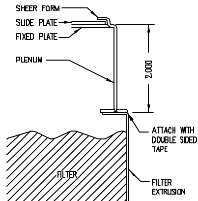
5 ENLARGED DETAIL
