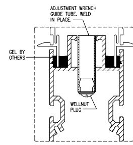
DAMPER ADJUSTMENT ACCESS HOLE PLUG
