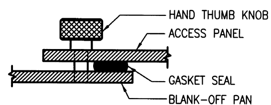
① ENLARGED SECTION
